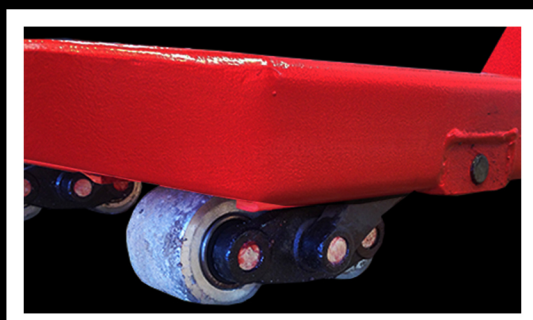
TANDEM STEEL LOAD ROLLERS WITH GUIDE ROLLERS
